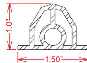
SMRP SECTION VIEW
