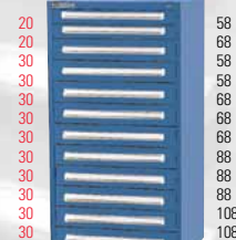
SEP3047AL 12 Drawers 224 Compartments 628 lbs. (285kg) Shipping Weight
