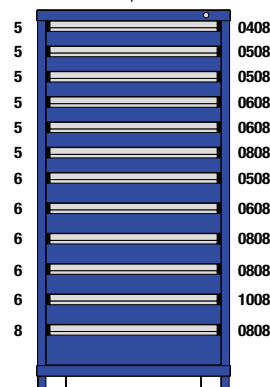
M1-302968FT-MD12CL 12 Drawers 240 Compartments
