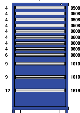
M1-302968FT-MD12EL 12 Drawers 214 Compartments
