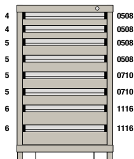
M1-232940FT-MD08AL 8 Drawers 90 Compartments
