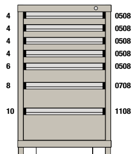
M1-232940FT-MD07AL 7 Drawers 100 Compartments
