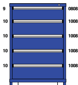
M1-302949FT-MD05AL 5 Drawers 64 Compartments
