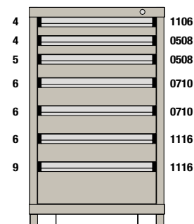
M1-232940FT-MD07BL 7 Drawers 86 Compartments
