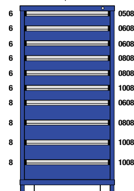
M1-302968FT-MD10DL 10 Drawers 168 Compartments
