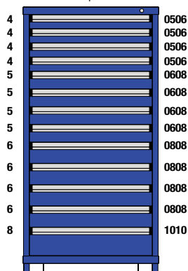
M1-302968FT-MD13BL 13 Drawers 273 Compartments
