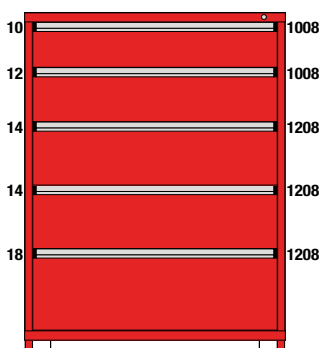
M1-452968FT- MD05AL 5 Drawers 88 Compartments
