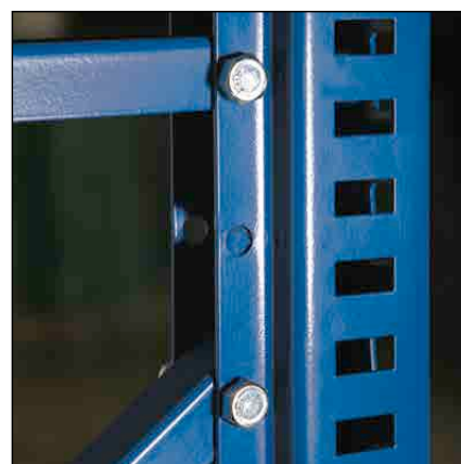
Ready-To-Assemble (bolt together) frame shown
