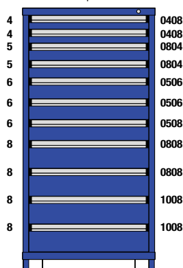
M1-302968FT-MD11AL 11 Drawers 268 Compartments
