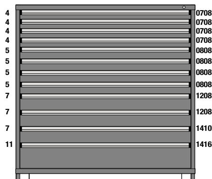
M1-602968FT-MD12BL 12 Drawers 377 Compartments
