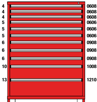
M1-452968FT-MD11AL 11 Drawers 317 Compartments
