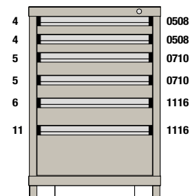
M1-232935FT-MD06CL 6 Drawers 58 Compartments
