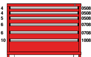
M1-452935FT-MD06AL 6 Drawers 204 Compartments
