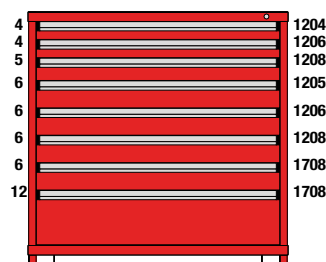
M1-452949FT-MD08AL 8 Drawers 152 Compartments
