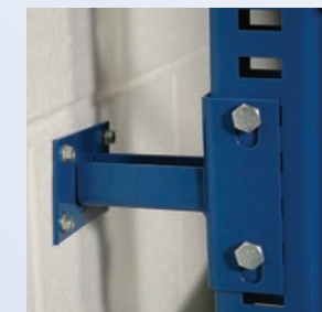
Wall ties anchor frames to wall and maintain adequate distance to allow beam adjustment.
