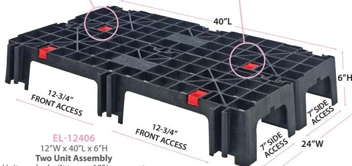
LOCKING SYSTEMS Simple locking system allows for quick and trouble-free assembly
